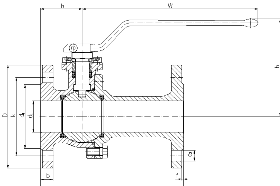
Picture 2: Ball valve with full bore flange acc. To DIN EN 1092-1 form B1; face to face dimension row 28 acc. to DIN EN 558-1 (F17 (long) acc. to DIN 3202 part 1)
