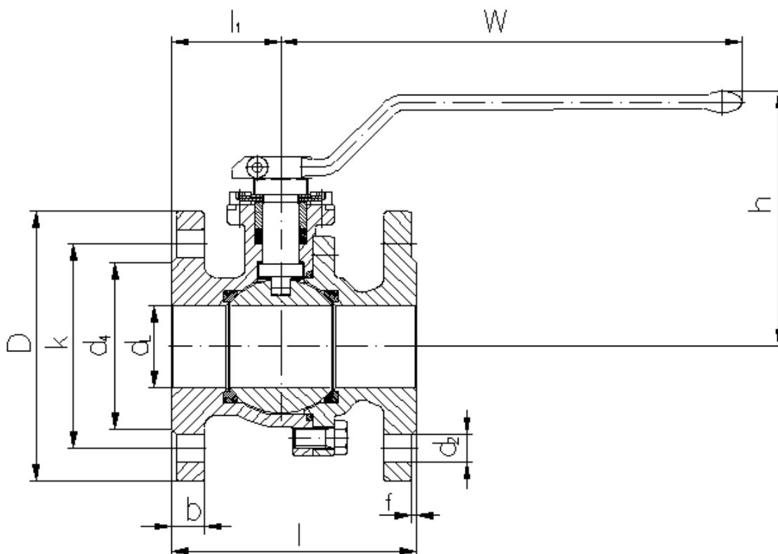
Picture 3: full bore ball valve with connection flange acc. to DIN EN1092-1 form B1; face to face length row 27 acc.to EN 558-1 (F18 acc. to DIN 3202 part 1)
